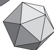
icosaedro regular
