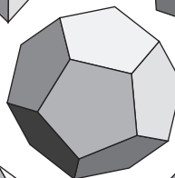
dodecaedro regular
