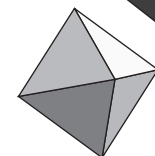
octaedro regular
