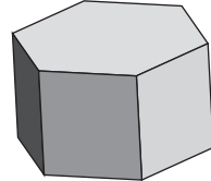
prisma hexagonal
