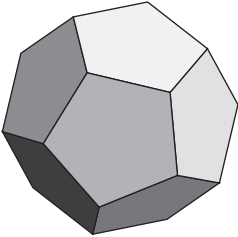
dodecaedro regular
