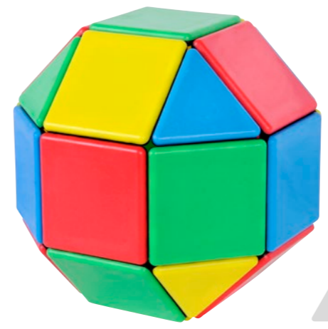
Small Rhombicuboctahedron
