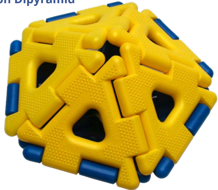
Pentagon Dipyramid
